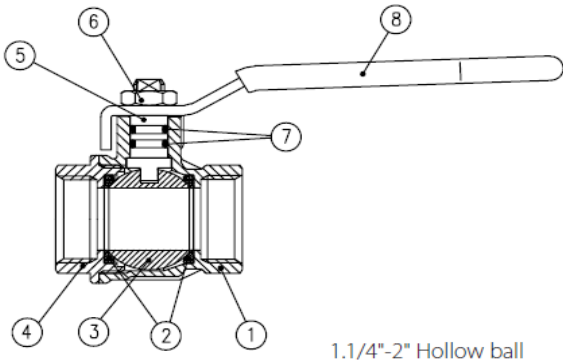
1.1/4"-2" Hollow ball
