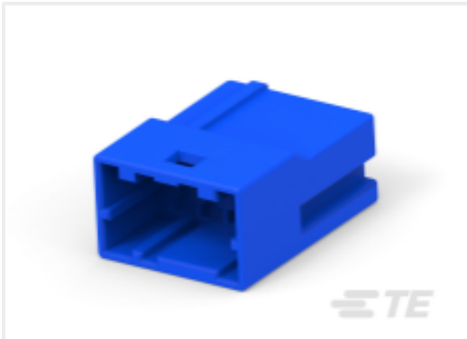
TE Part #2-2232574-3 GIC 2.5 W CAP HSG 4P BLUE
