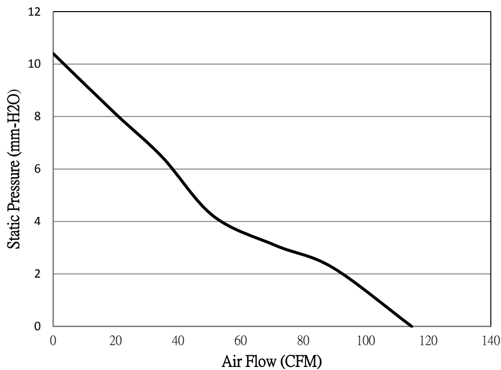
P-Q Curve
