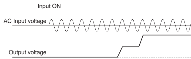
Fig. 2.1 Start-up waveform for series and parallel operation
