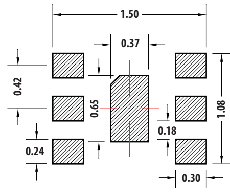
Stencil Opening
