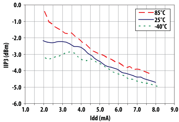
Figure 17. IIP3 vs Idd over temperature at Vdd=1.8V
