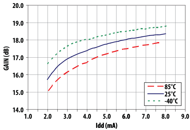
Figure 15. Gain vs Idd over temperature at Vdd=1.8V
