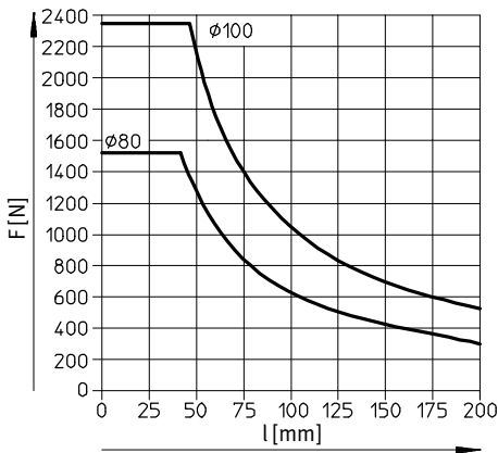
DFM-80 ... 100-GF Hub 50 mm
