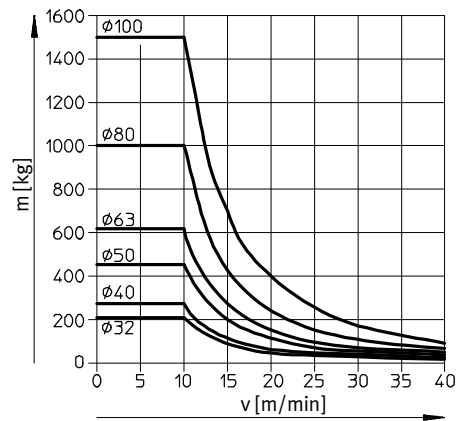
DFM-32 ... 100-GF Hub < 50 mm
