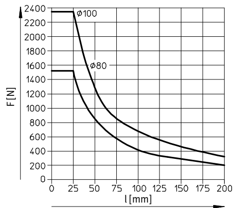
DFM-80 ... 100-KF Hub 80 ... 200 mm
