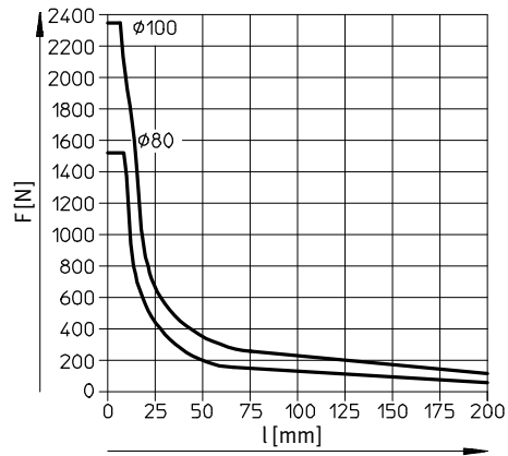
DFM-80 ... 100-KF Hub 25 mm
