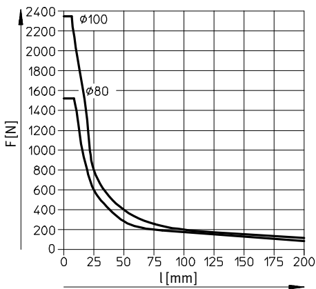
DFM-80 ... 100-KF Hub 50 mm
