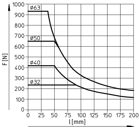
DFM-32 ... 63-KF Hub 125 ... 200 mm
