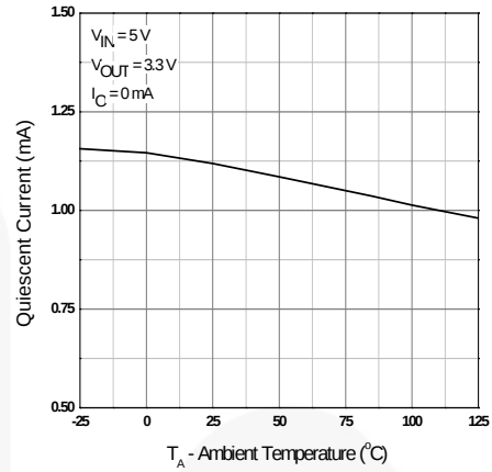
Figure 4. Quiescent vs. Temperature
