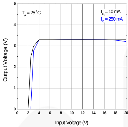
Figure 9. Output Voltage vs. Input Voltage
