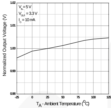
Figure 3. Normalized Output Voltage
