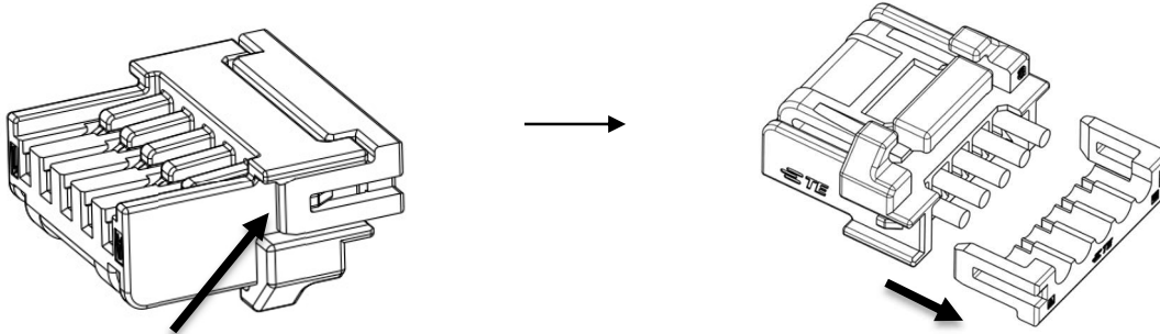
Single Row
