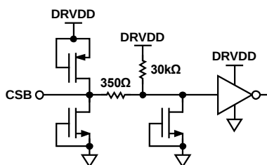
Figure 15. CSB
