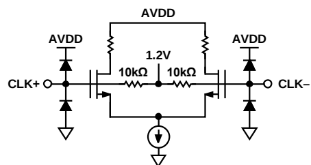
Figure 13. Clock Inputs
