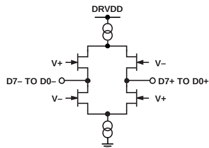
Figure 18. LVDS Output Driver
