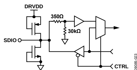
Figure 17. SDIO
