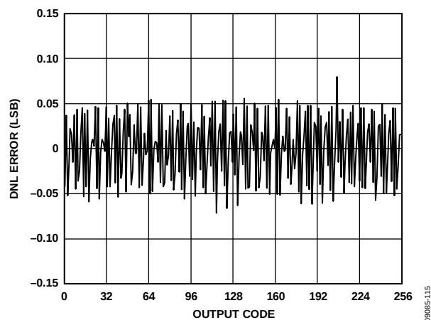
Figure 11. DNL Error with f_{IN} = 4.3 MHz
