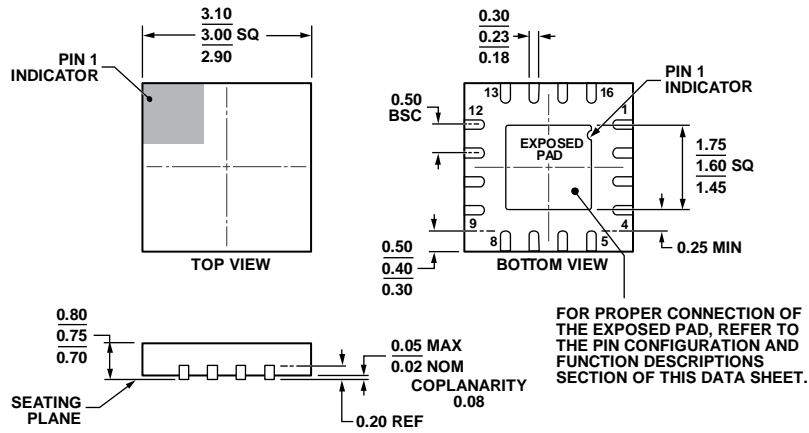
Figure 46. 16-Lead Lead Frame Chip Scale Package [LFCSP_WQ] 3 mm × 3 mm Body, Very Very Thin Quad (CP-16-22)
