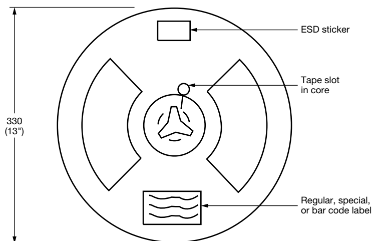
Fig. 19 - Reel Dimensions (550 units per reel)
