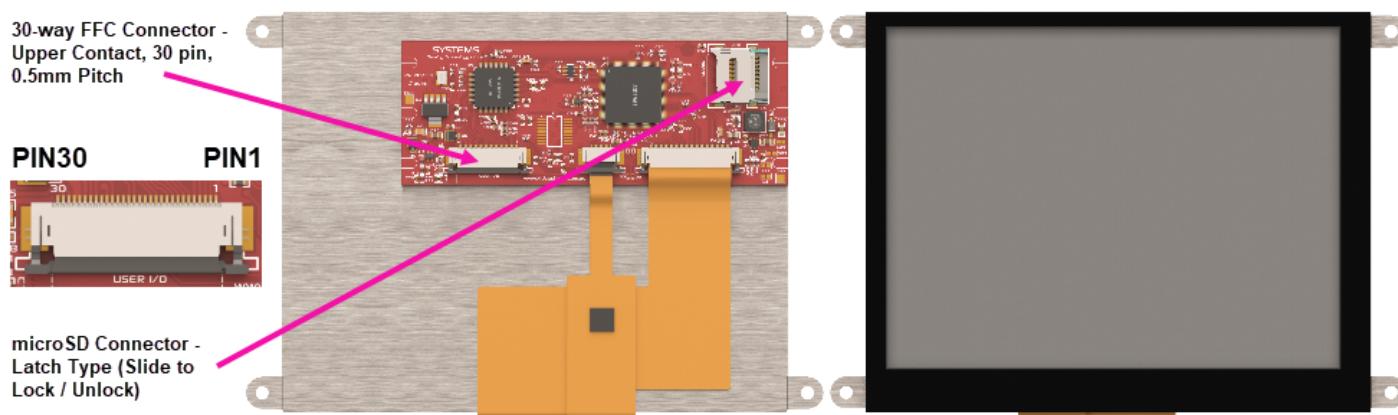
FFC Pinout
