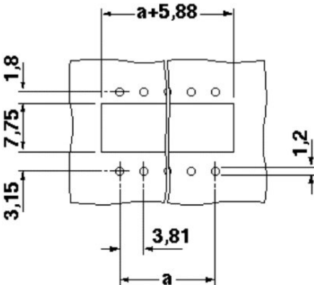
Drilling diagram
