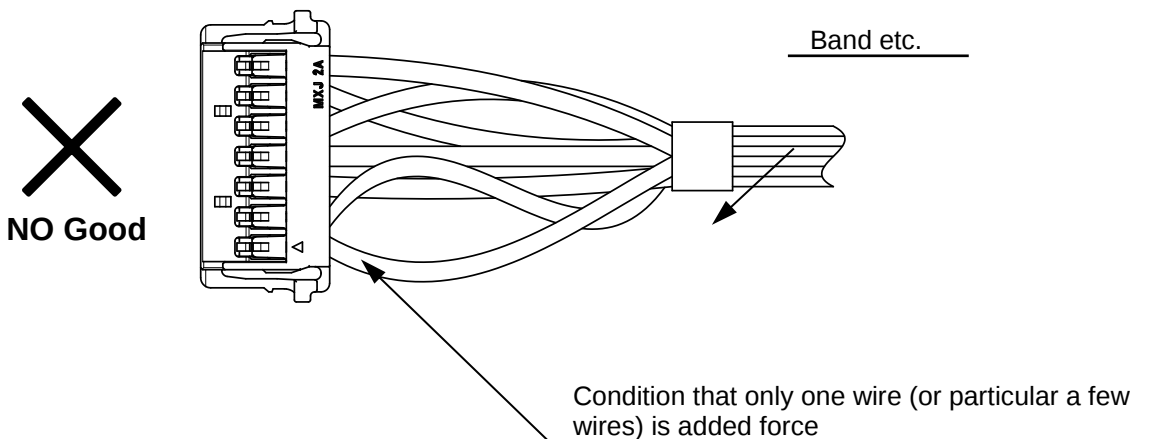
Fig.7-2 Condition that harness is banding improperly
