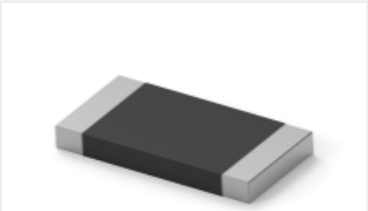
TE Part #8-2176422-0 TLRP 2512 3.0W R200 1% 50PPM 4K RL
