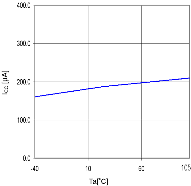
Figure 22. T_a - I_{CC}
