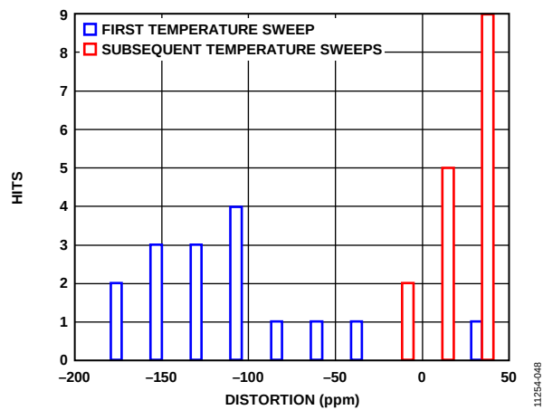
Figure 45. Thermal Hysteresis
