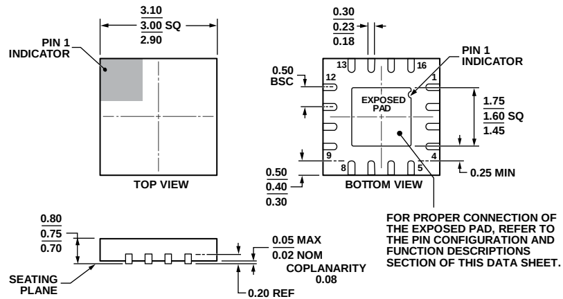
Figure 50. 16-Lead Lead Frame Chip Scale Package [LFCSP_WQ] 3 mm × 3 mm Body, Very Very Thin Quad (CP-16-22) Dimensions shown in millimeters
