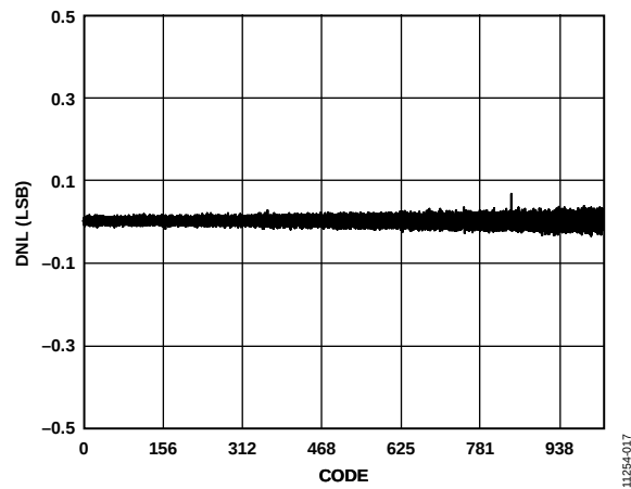
Figure 15. Differential Nonlinearity (DNL) vs. Code
