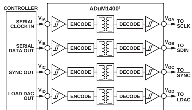
Figure 49. Isolated Interface
