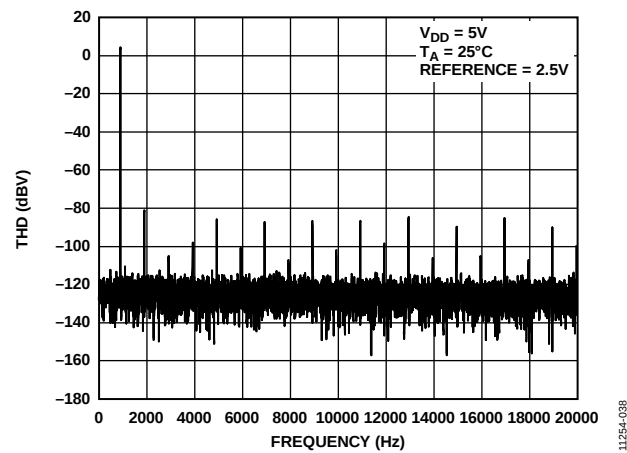
Figure 36. Total Harmonic Distortion at 1 kHz
