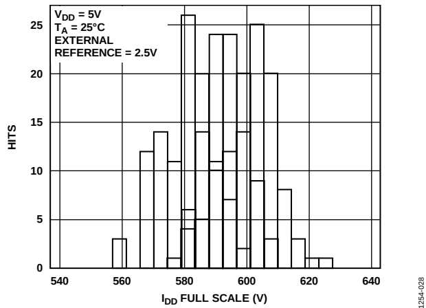
Figure 26. I_{DD} Histogram with External Reference, V_{DD} = 5 V
