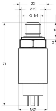
CH2 Connector
