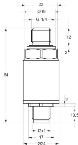
CN5A: M12, 5 Pin Connector Output
