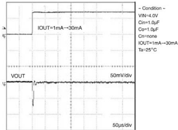
Figure 9. Load response
