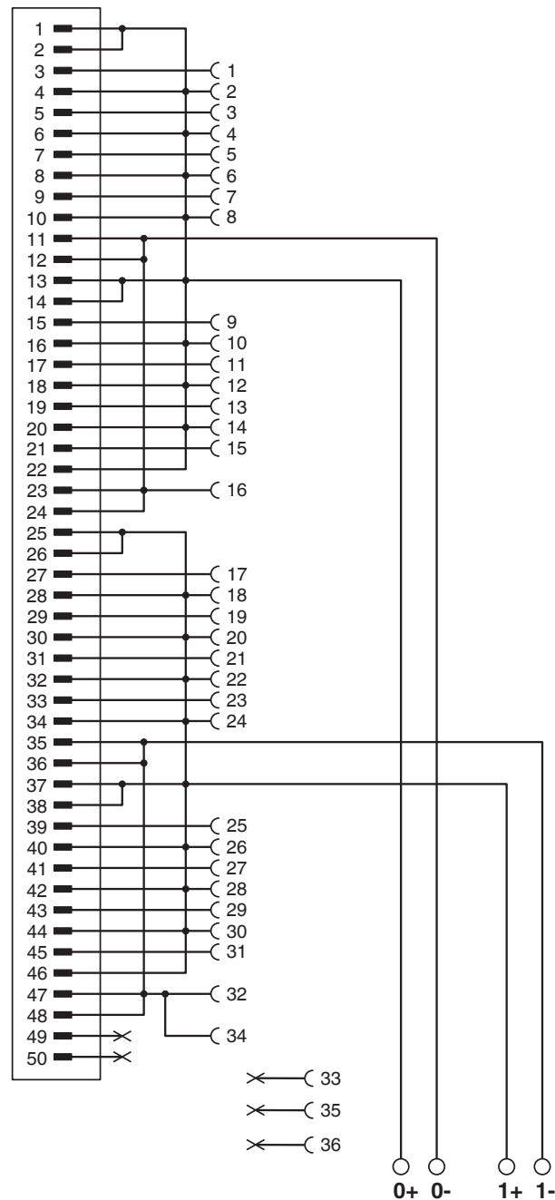
Circuit diagram
