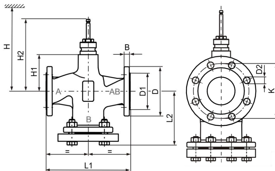
Valve, DN150
