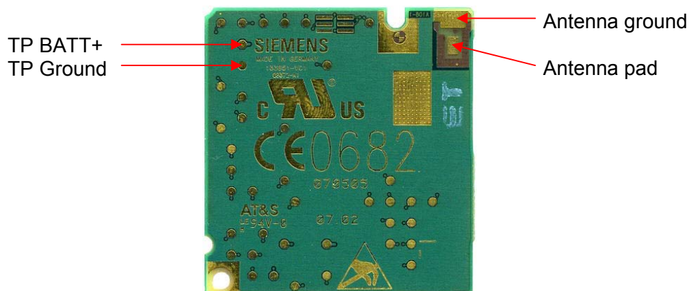
Figure 44: MC55/56 bottom view
