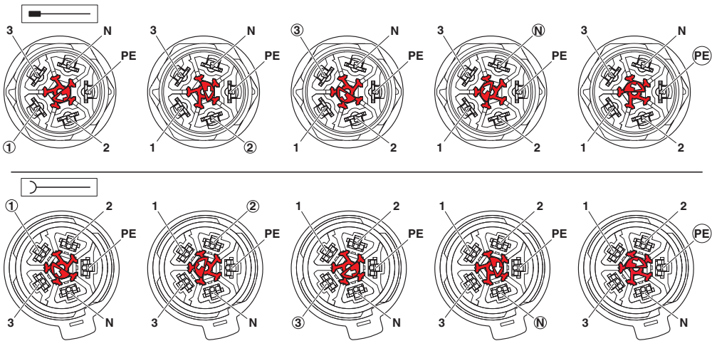
Functional drawing
