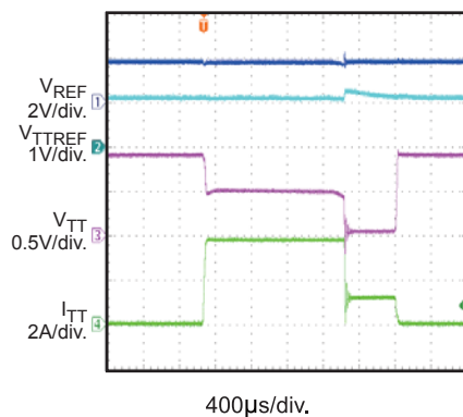
Source Over Current Protection
