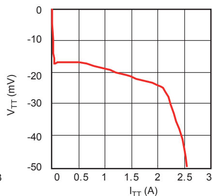
DDR2 Source Regulation
