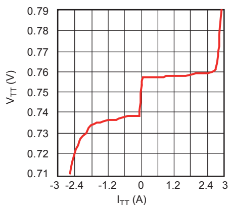
DDR3 Regulation
