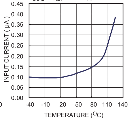
Shut Down Input Current vs. Temp
