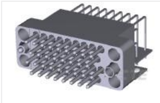
TE Part #213289-2 V.35,PIN ASY,RA,34P,W/BRKT LF
