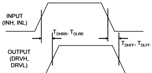
Figure 1—Timing Diagram
