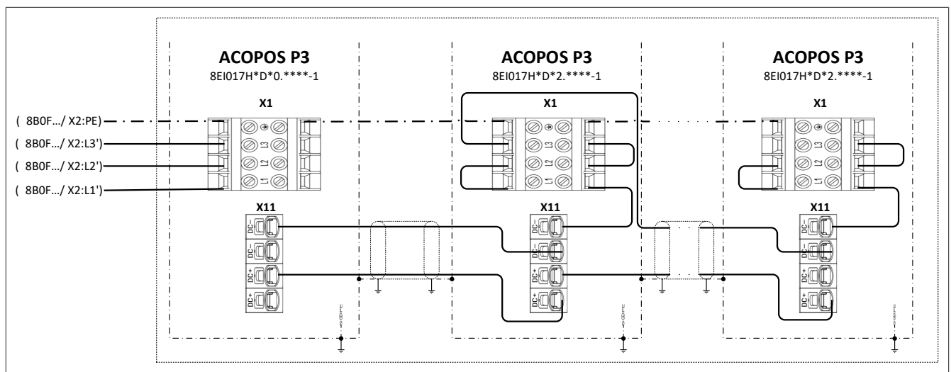
Figure 5: DC bus network
