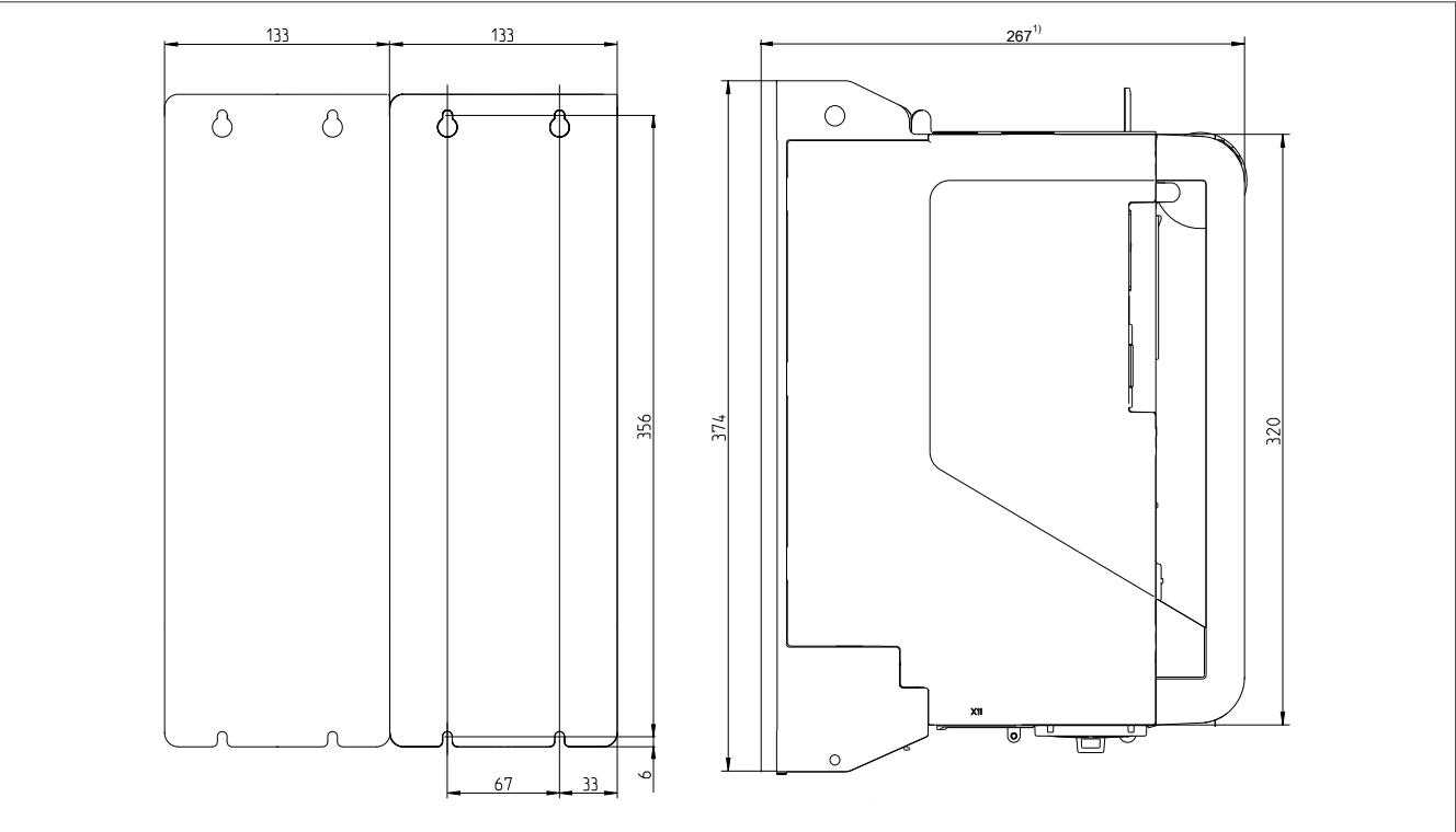
Figure 2: Dimension diagram for double-width modules
