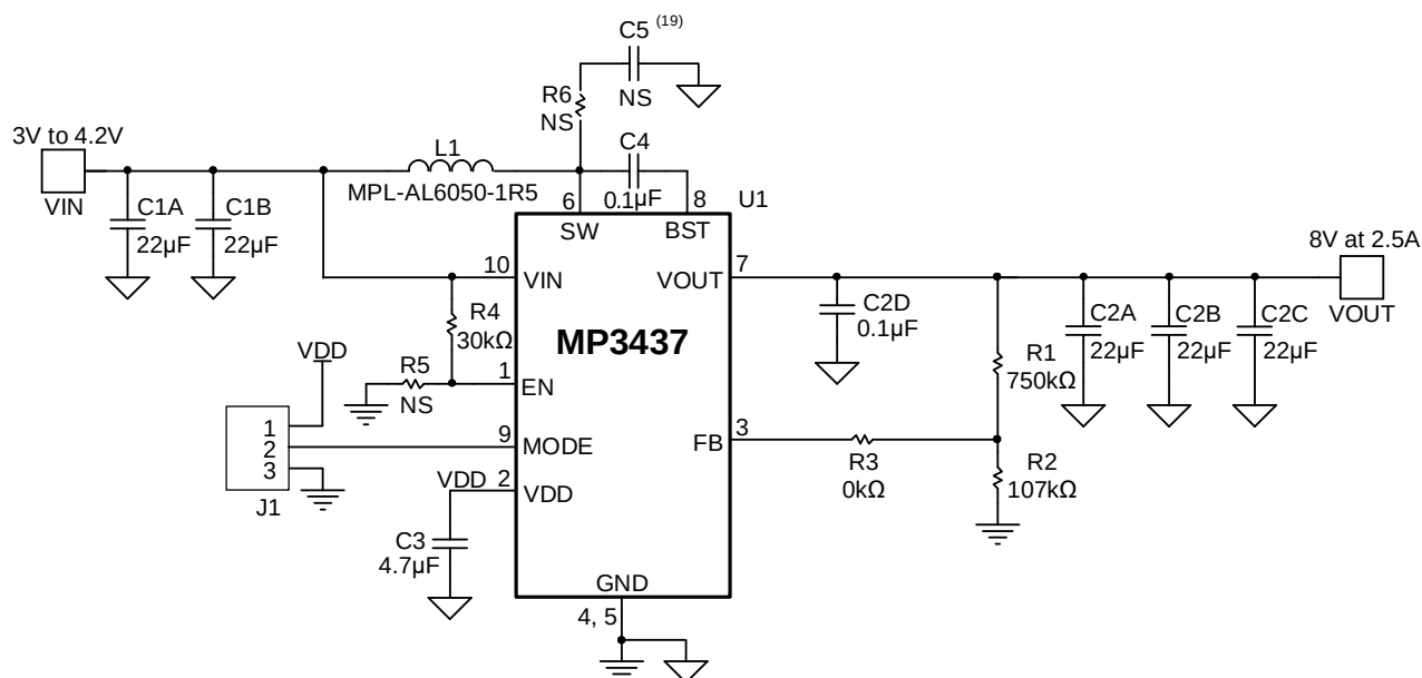
Figure 5: QFN Package Typical Application Circuit
