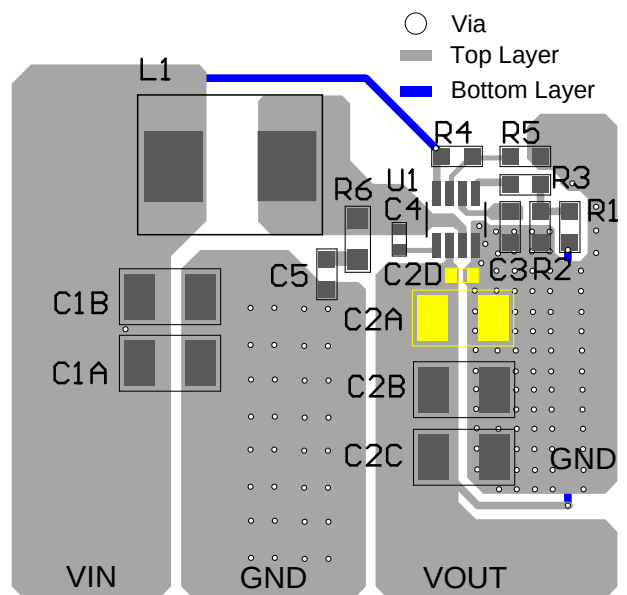
Figure 4: Recommended PCB Layout for TSOT23 Package
