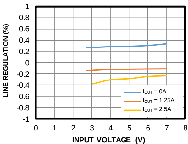
Line Regulation
