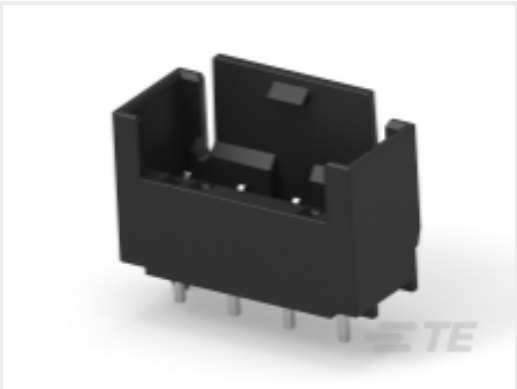
TE Part #4-2232199-7 4/7P,RAST 2.5 Tab Header,Ex- Locking, THV
