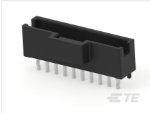
TE Part #5-2232826-0 SGI2.0 header assembly TH 10P,key B, BLK
