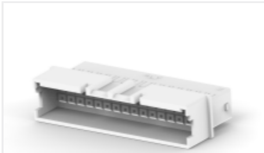
TE Part # 3-2324201-2 HSG,REC,FREE-HANGING,GWT, DUALROW,EP2.5
