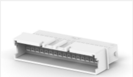
TE Part # 1-1969567-0 HOUSING, PLUG, GWT, DUAL ROW, EP2.5
