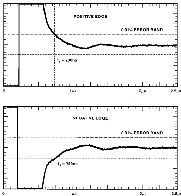
FIGURE 5: OP-42 Settling-Characteristics optimal settling speed. Compensation is achieved with ca-
