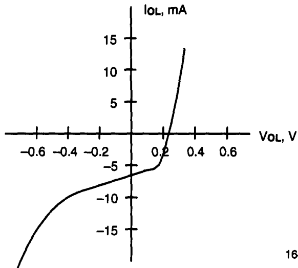
Output, LOW
