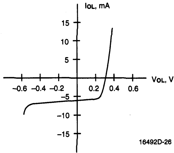
Output, LOW
