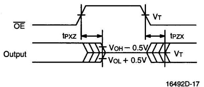
OE to Output Disable/Enable
