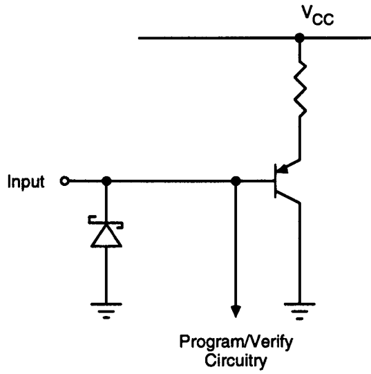
Typical Input
