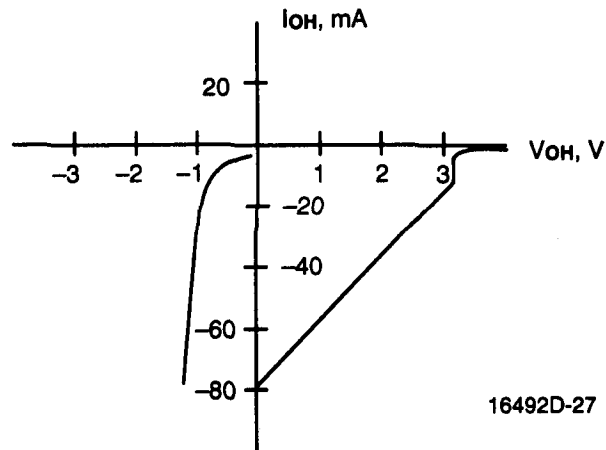
Output, HIGH
