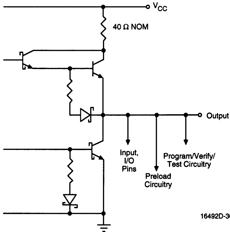
Typical Output
