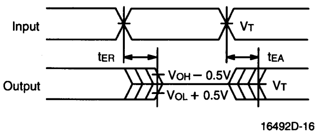
Input to Output Disable/Enable
