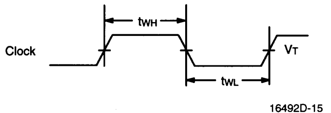
Clock Width
