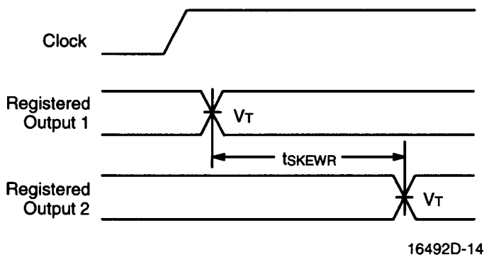
Registered Output Skew
