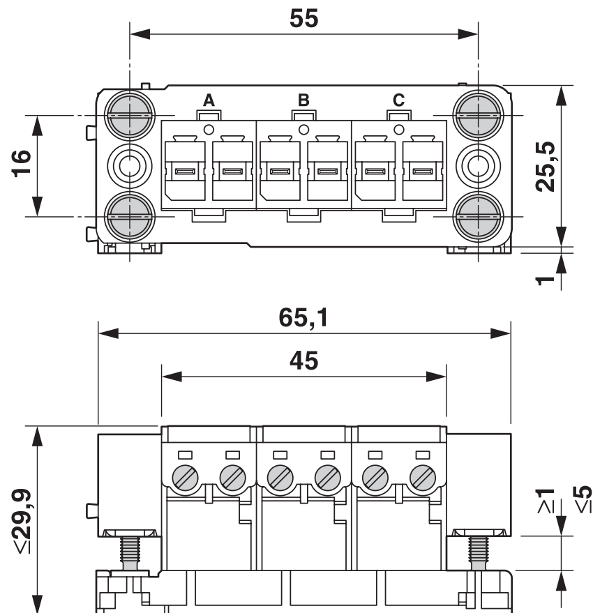
Dimensional drawing
