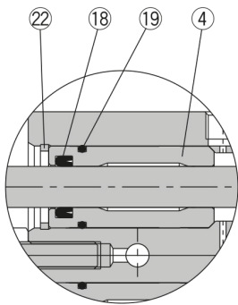
Rod cover
