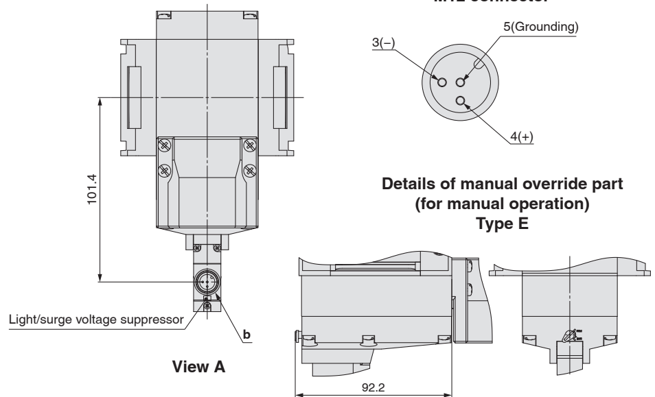
Detailed figure of b section M12 connector
