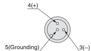
Detailed figure of b section M12 connector
