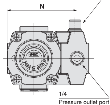
M12 x 1 Power cable connection thread (Plug type)
