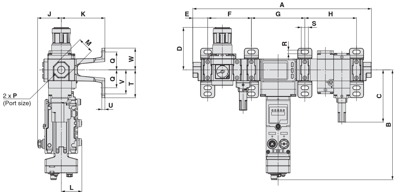
AMS20/30/40/60B-□00D (Without attachments)
