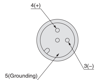
Detailed figure of b section M12 connector
