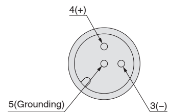
Detailed figure of b section M12 connector
