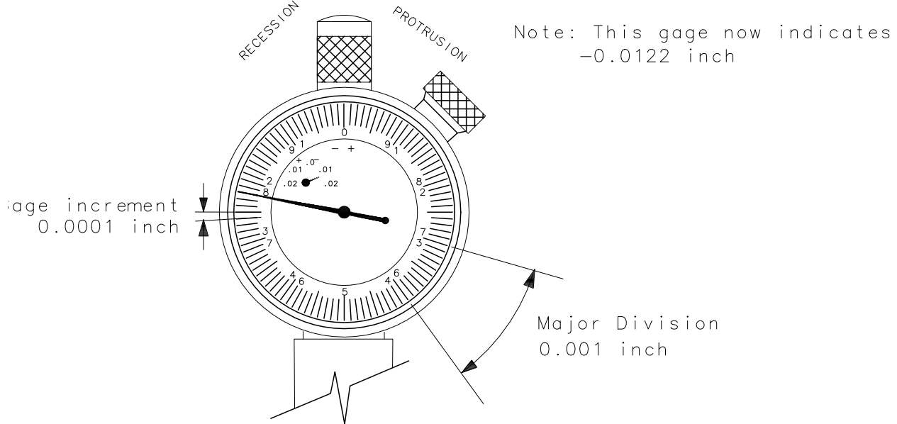
Figure 3-2 Reading the Connector Gage
