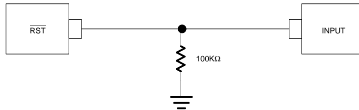
\overline{RST} VALID TO 0 VOLTS V_{CC} Figure 8
