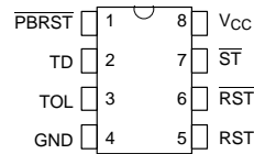
DS1832 8-PIN DIP (300 MIL) See Mech. Drawings Section
