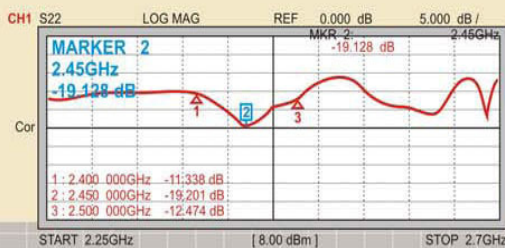
Return Loss
