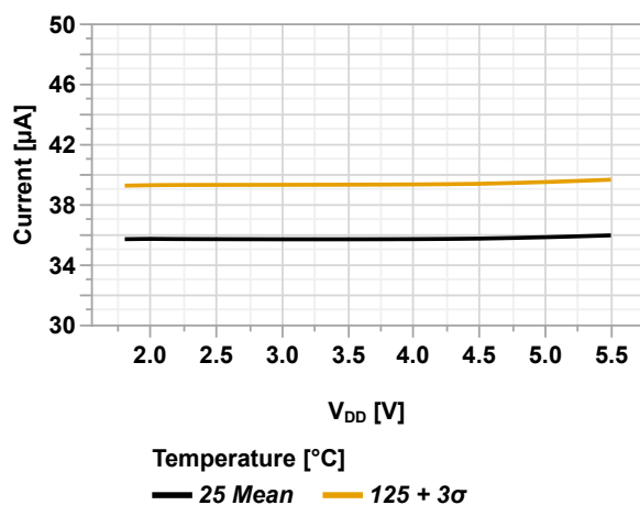
Figure 49-30. I_{PD} HLVD vs. V_{DD}
