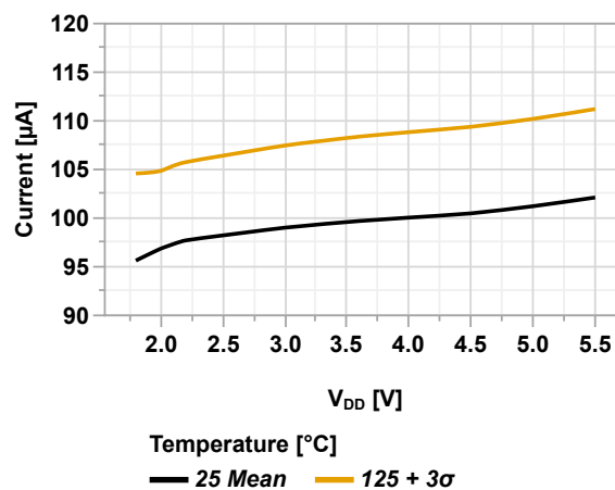
Figure 49-29. I_{PD} CMP (SP[1:0] = 0x3) vs. V_{DD}
