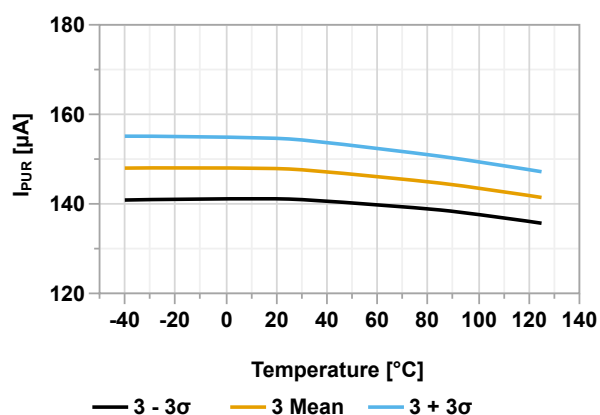
Figure 49-74. Weak Pull-up Current V_{SS} Temperature at V_{DD} = 3.0V
