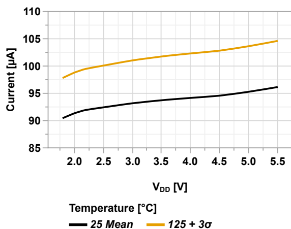
Figure 49-26. I_{PD} CMP (SP[1:0] = 0x0) vs. V_{DD}
