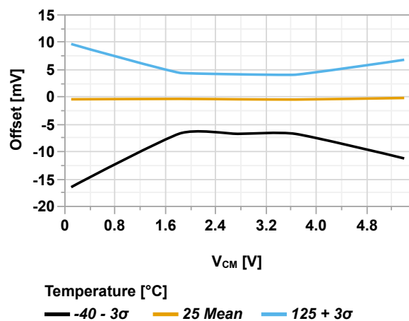
Figure 49-111. Input Offset vs. Common Mode Voltage ( V_{DD} = 5.5V )
