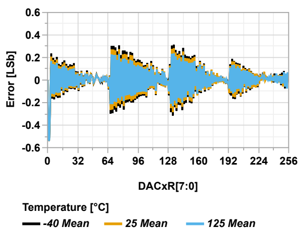
Figure 49-117. DNL vs. DAC Code ( V_{REF} = V_{DD} = 3.0V )
