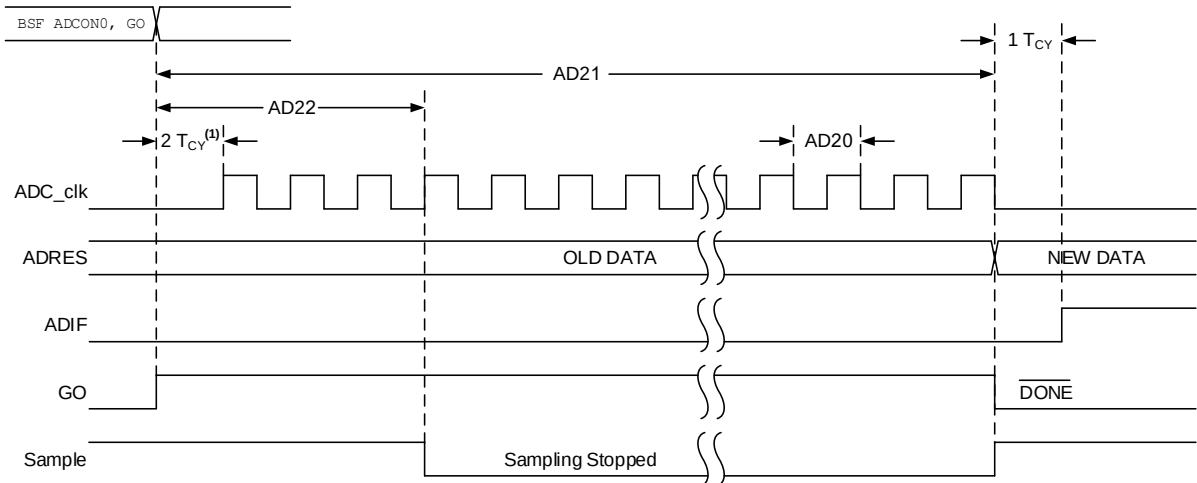
Figure 48-10. ADC Conversion Timing (ADC Clock from ADCRC)
