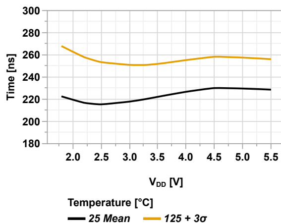
Figure 49-102. Falling Edge Response Time vs. V_{DD} ( V_{CM} = V_{DD}/2 , SP[1:0] = 0x3)
