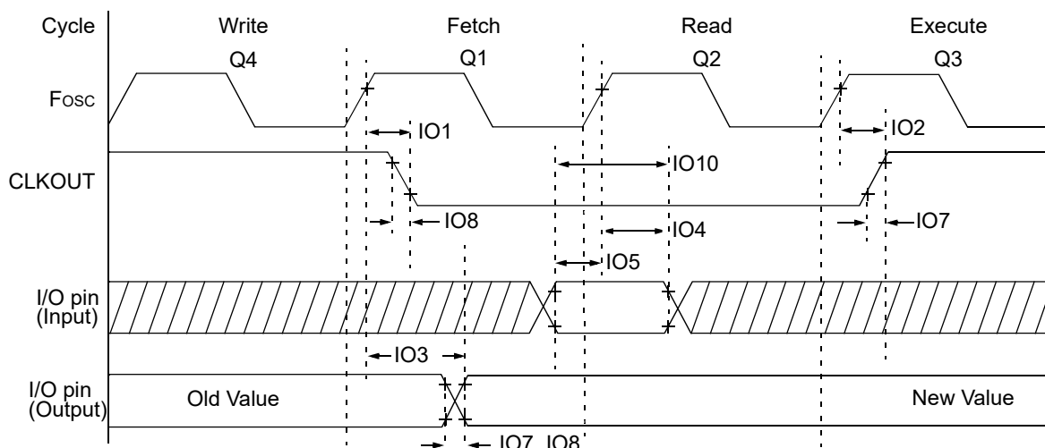
Figure 48-6. CLKOUT and I/O Timing
