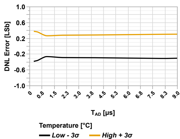
Figure 49-96. DNL vs. T_{AD} ( V_{REF+} = V_{DD} = 3.0V , T = 125^{\circ}C , CPON = 1 )
