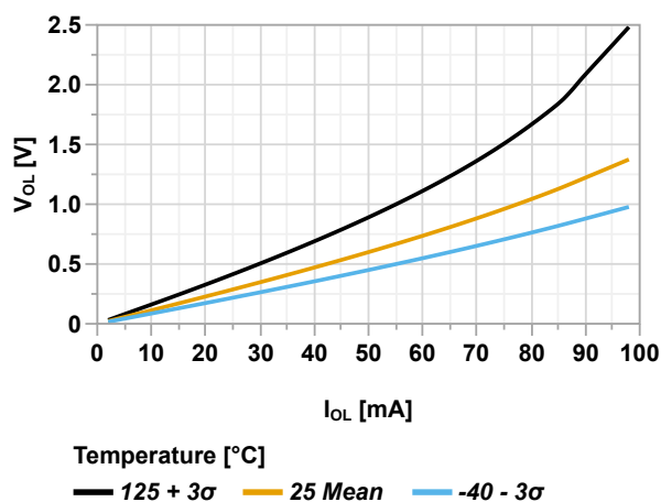
Figure 49-80. Output Pin - Maximum V_{OL} vs. Current, V_{DD} = 5.5V
