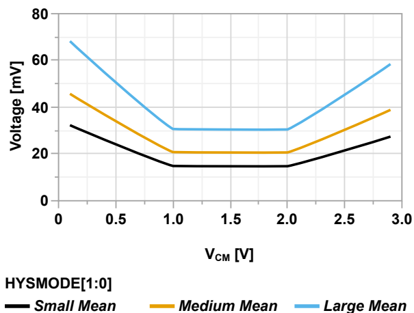
Figure 49-110. Input Hysteresis vs. Common Mode Voltage ( V_{DD} = 3.0V )
