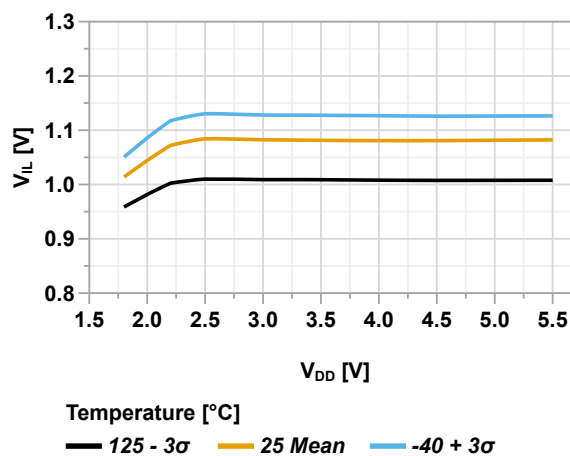
Figure 49-69. Input Pin with SMBus - Maximum V_{IL} vs. V_{DD}
