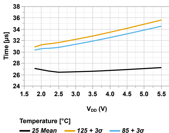
Figure 49-37. Wake-up Time (COSC[2:0] = 'b110, OSCFRQ = 4 MHz, VREGPM[1:0] = 'b01 = LP) vs. V_{DD}
