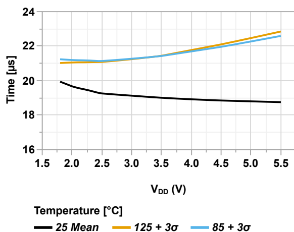
Figure 49-39. Wake-up Time (COSC[2:0] = 'b110, OSCFRQ = 4 MHz, VREGPM[1:0] = 'b00 = HP) vs. V_{DD}
