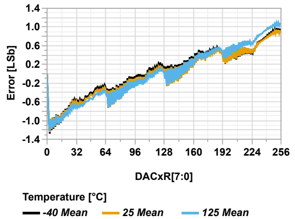
Figure 49-120. INL vs. DAC Code ( V_{REF} = V_{DD} = 5.5V )
