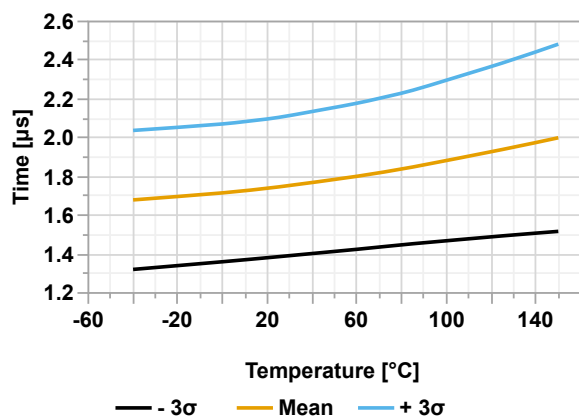
Figure 49-56. BOR Response Time vs. Temperature
