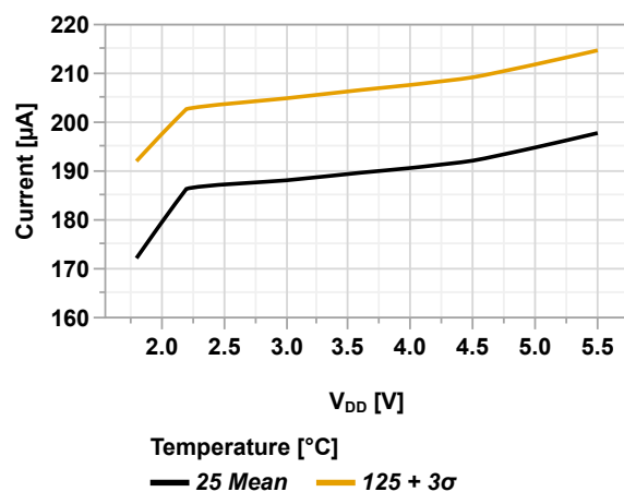
Figure 49-22. I_{PD} ADFVR vs. V_{DD}
