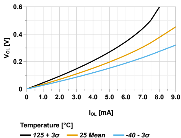
Figure 49-78. Output Pin - Maximum V_{OL} vs. Current, V_{DD} = 3.0V
