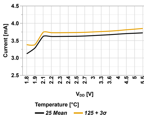
Figure 49-8. Active Power Consumption vs. V_{DD} (RSTOSC[2:0] = 'b111, FEXTOSC[3:0] = 'b0011, HS = 16 MHz, PMDx = 0xFF)
