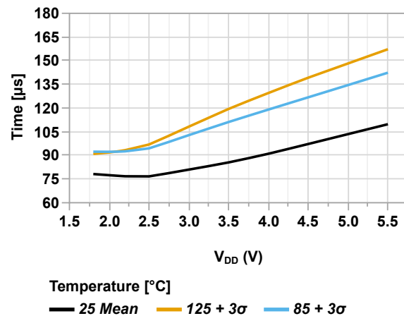
Figure 49-34. Wake-up Time (COSC[2:0] = 'b110, OSCFRQ = 4 MHz, VREGPM[1:0] = 'b10 = ULP) vs. V_{DD}
