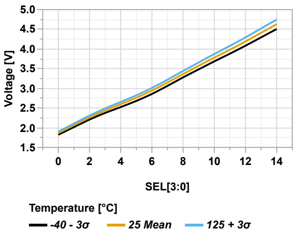
Figure 49-59. HLVD Positive Edge SEL[3:0] vs. Temperature
