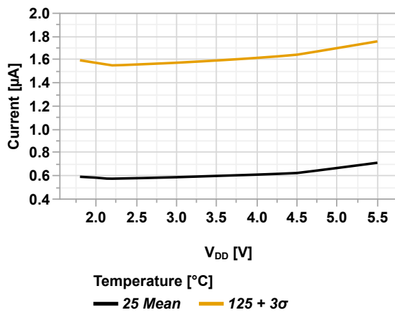
Figure 49-14. I_{PD} Base (VREGPM[1:0] = 'b11 = ULP + Extended Temperature Range) vs. V_{DD}
