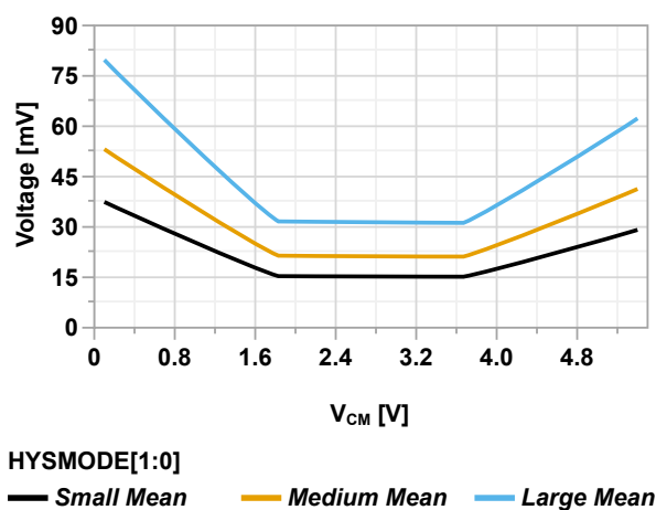
Figure 49-112. Input Hysteresis vs. Common Mode Voltage ( V_{DD} = 5.5V )
