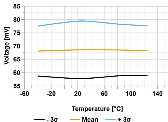
Figure 49-53. BOR Hysteresis (BORV[1:0] = 0x1) vs. Temperature
