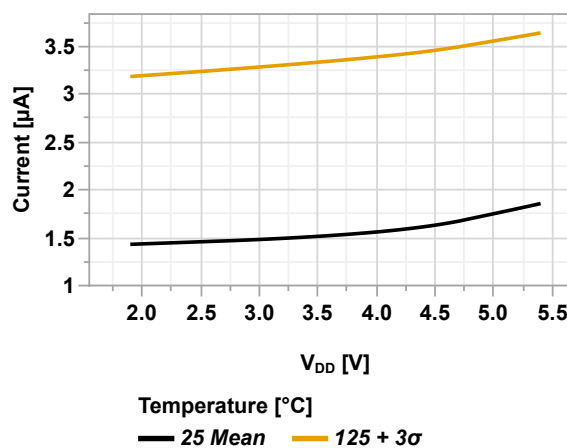
Figure 49-19. I_{PD} SOSC (SOSCPWR = Low Power) vs. V_{DD}
