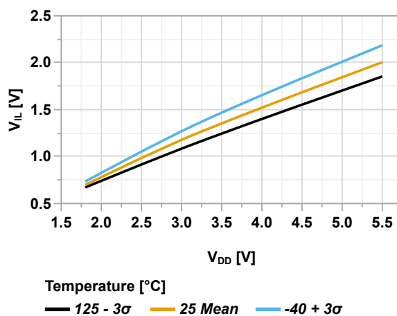
Figure 49-71. Reset Pin V_{IL} vs. V_{DD}
