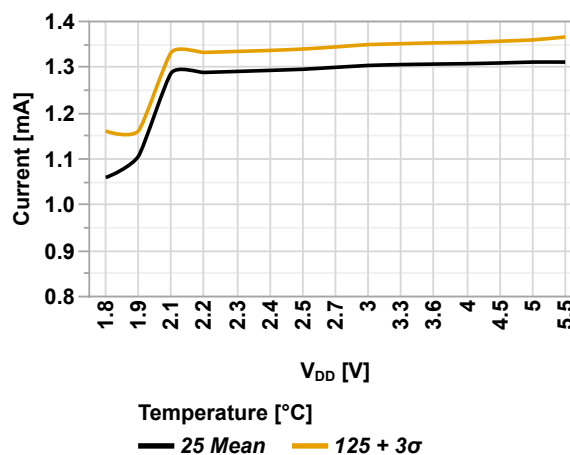
Figure 49-12. Doze Power Consumption vs. V_{DD} (RSTOSC[2:0] = 'b110, OSCFRQ = 16 MHz)
