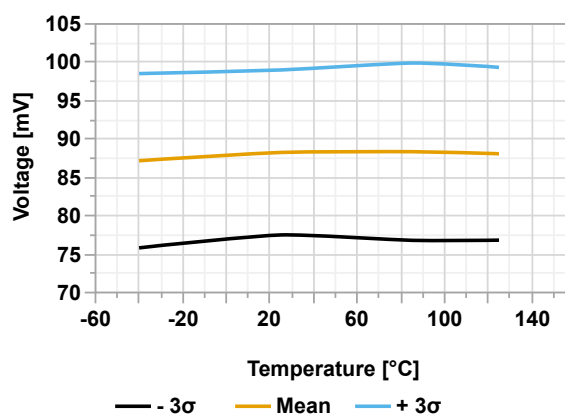
Figure 49-55. BOR Hysteresis (BORV[1:0] = 0x3) vs. Temperature
