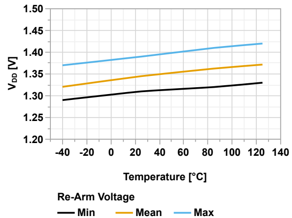
Figure 49-47. POR Re-Arm Voltage vs. Temperature
