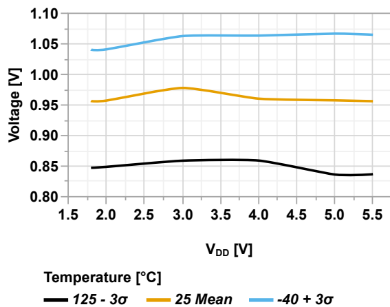
Figure 49-125. Zero-Cross Detector Trip Voltage vs. V_{DD}
