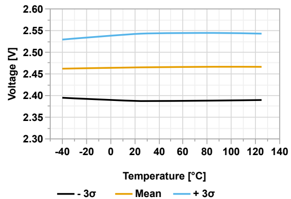
Figure 49-49. BOR Threshold Level (BORV[1:0] = 0x1) vs. Temperature
