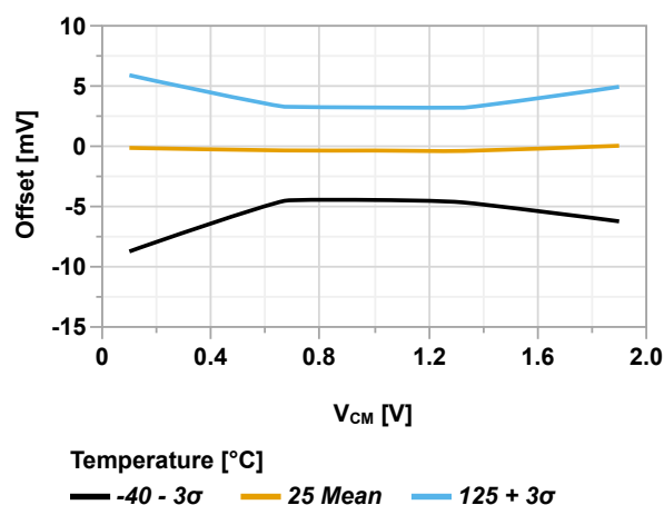
Figure 49-109. Input Offset vs. Common Mode Voltage ( V_{DD} = 3.0V )
