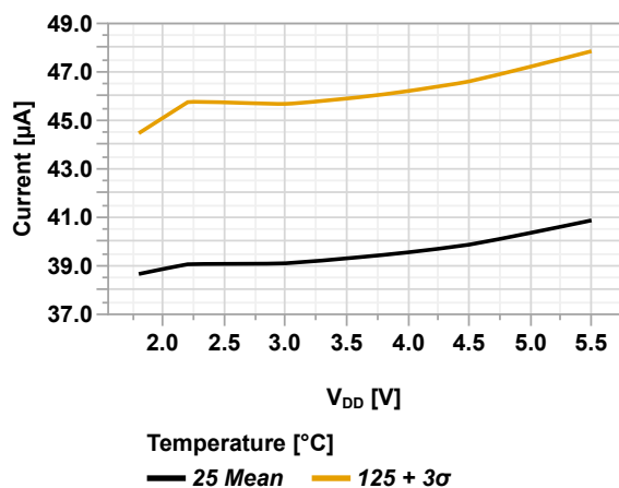
Figure 49-18. I_{PD} WDT vs. V_{DD}
