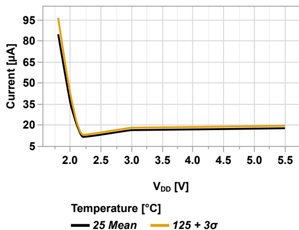
Figure 49-26. I_{PD} CMP (SP[1:0] = 0x0) vs. V_{DD}
