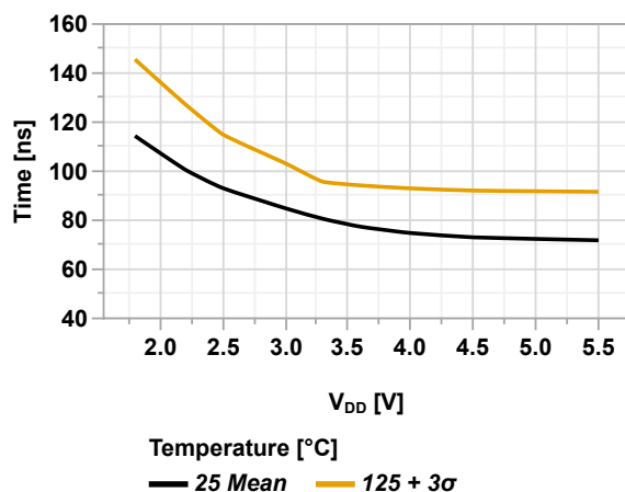
Figure 49-105. Rising Edge Response Time vs. V_{DD} ( V_{CM} = V_{DD}/2 , SP[1:0] = 0x2)
