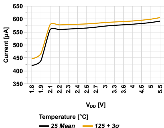
Figure 49-3. Active Power Consumption vs. V_{DD} (RSTOSC[2:0] = 'b110, OSCFRQ = 16 MHz, PMDx = 0x00)
