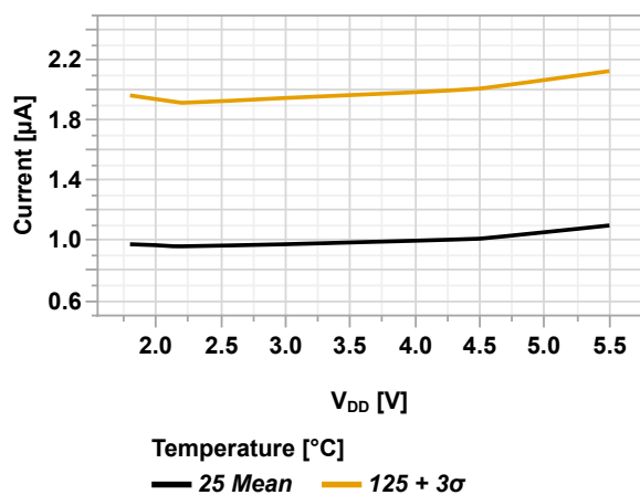
Figure 49-18. I_{PD} WDT vs. V_{DD}
