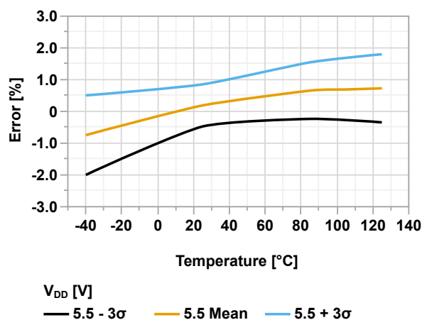
Figure 49-83. ADFVR Voltage Error vs. Temperature ( V_{DD} = 5.5V , V_{REF} = 2.048V )
