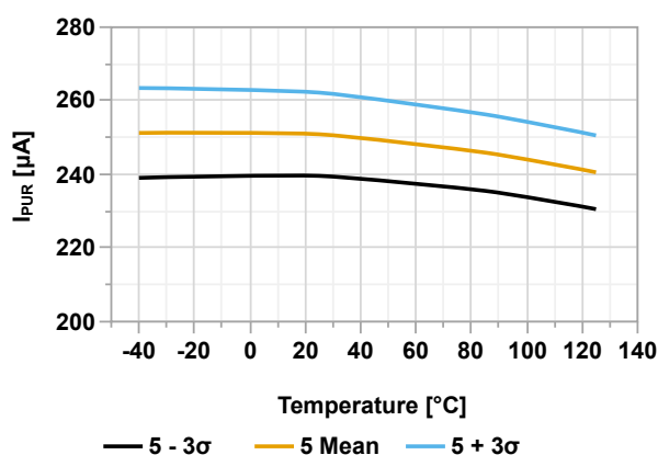
Figure 49-75. Weak Pull-up Current V_{SS} Temperature at V_{DD} = 5.0V
