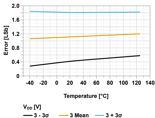
Figure 49-113. Gain Error vs. Temperature ( V_{REF} = V_{DD} = 3.0V )
