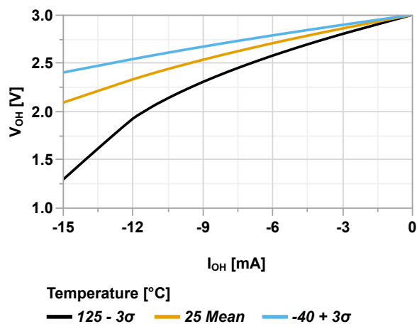
Figure 49-79. Output Pin - Minimum V_{OH} vs. Current, V_{DD} = 3.0V
