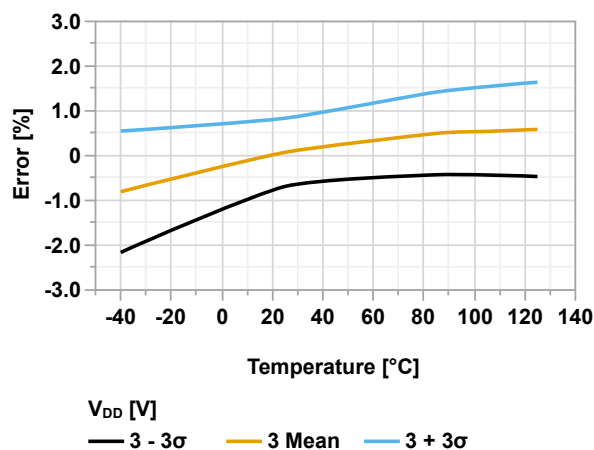
Figure 49-91. CDAFVR Voltage Error vs. Temperature ( V_{DD} = 3.0V , V_{REF} = 2.048V )
