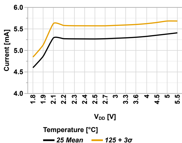
Figure 49-11. Idle Power Consumption vs. V_{DD} (RSTOSC[2:0] = 'b110, OSCFRQ = 16 MHz)
