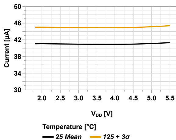
Figure 49-27. I_{PD} CMP (SP[1:0] = 0x1) vs. V_{DD}
