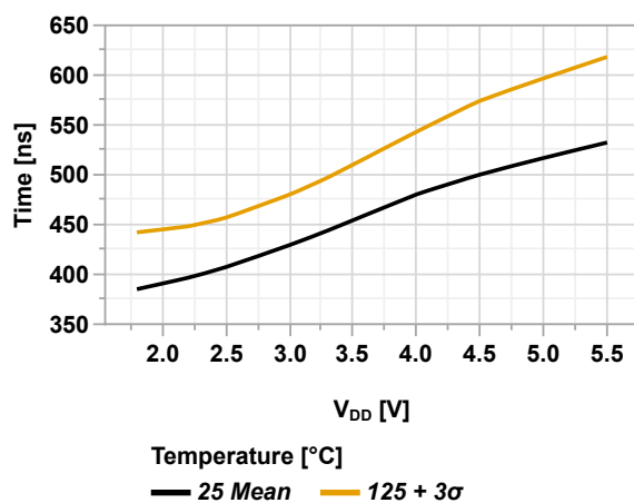
Figure 49-101. Falling Edge Response Time vs. V_{DD} ( V_{CM} = V_{DD}/2 , SP[1:0] = 0x2)
