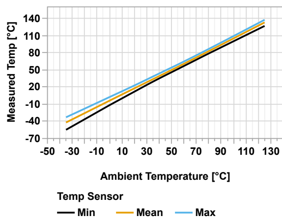
Figure 49-98. Temperature Sensor Characteristics, V_{DD} = 3.0V
