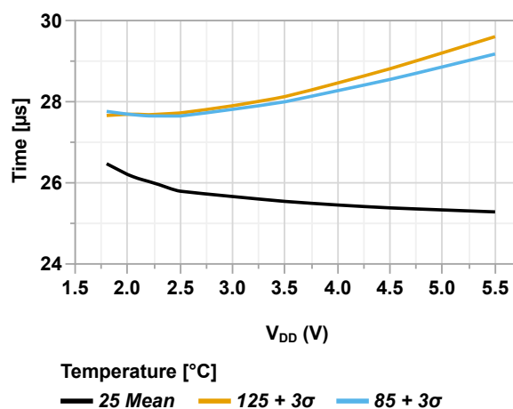
Figure 49-40. Wake-up Time (COSC[2:0] = 'b110, OSCFRQ = 16 MHz, VREGPM[1:0] = 'b00 = HP) vs. V_{DD}
