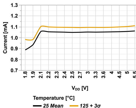
Figure 49-8. Active Power Consumption vs. V_{DD} (RSTOSC[2:0] = 'b111, FEXTOSC[3:0] = 'b0011, HS = 16 MHz, PMDx = 0xFF)
