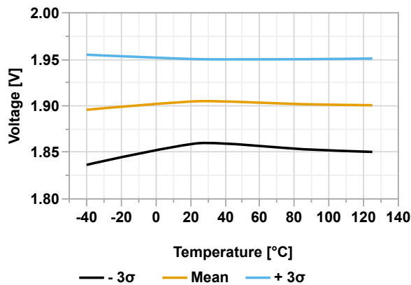
Figure 49-48. BOR Threshold Level (BORV[1:0] = 0x0) vs. Temperature
