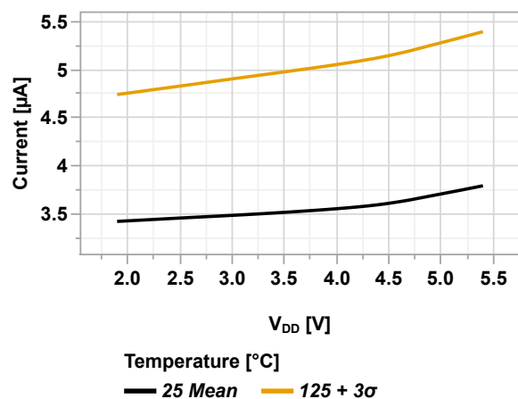
Figure 49-22. I_{PD} ADFVR vs. V_{DD}
