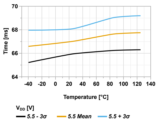
Figure 49-45. Start-up Time vs. Temperature (PWRTS[1:0] = 0x2, V_{DD} = 5.5V)
