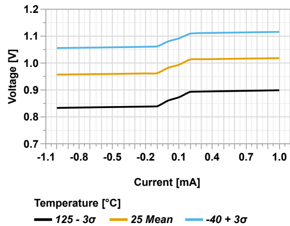
Figure 49-124. Zero-Cross Detector Pin Voltage vs. Current ( V_{DD} = 3.0V )
