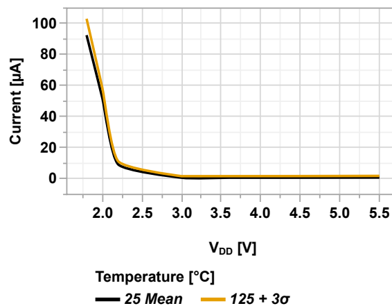
Figure 49-23. I_{PD} CDAFVR vs. V_{DD}
