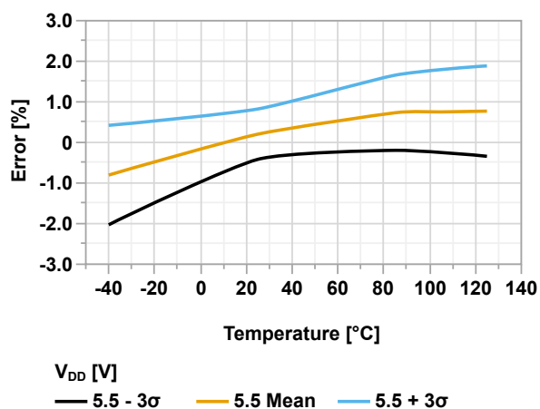
Figure 49-82. ADFVR Voltage Error vs. Temperature ( V_{DD} = 5.5V , V_{REF} = 1.024V )
