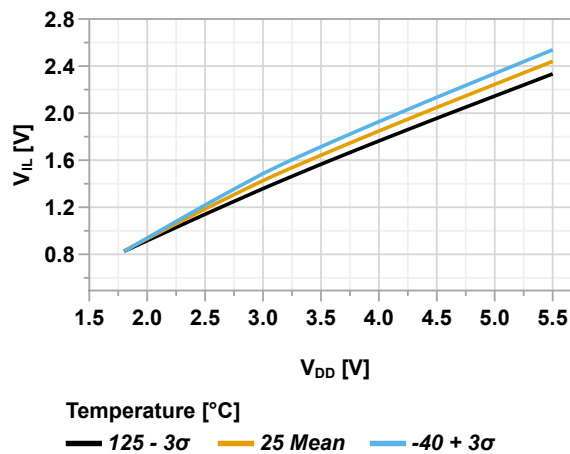
Figure 49-67. Input Pin with I 2 C Trigger - Maximum V_{IL} vs. V_{DD}
