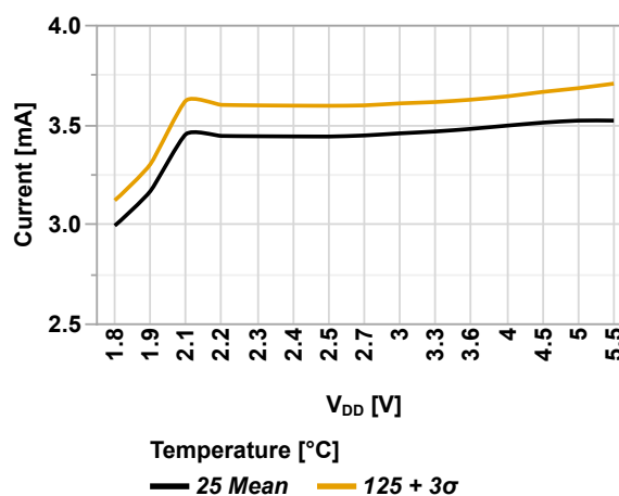
Figure 49-12. Doze Power Consumption vs. V_{DD} (RSTOSC[2:0] = 'b110, OSCFRQ = 16 MHz)
