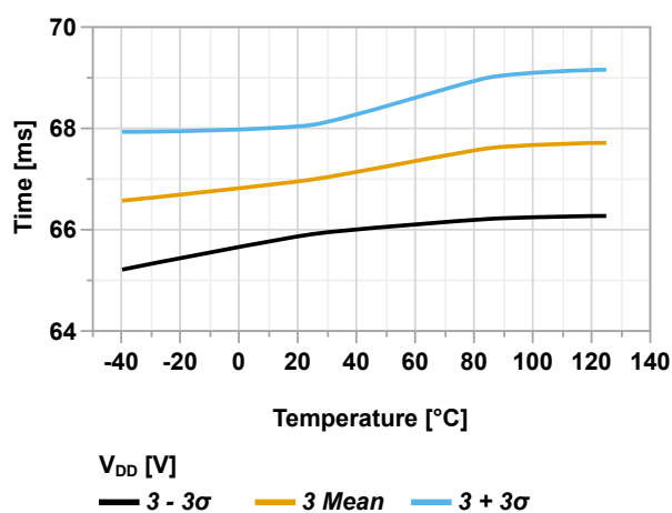
Figure 49-44. Start-up Time vs. Temperature (PWRTS[1:0] = 0x2, V_{DD} = 3.0V)
