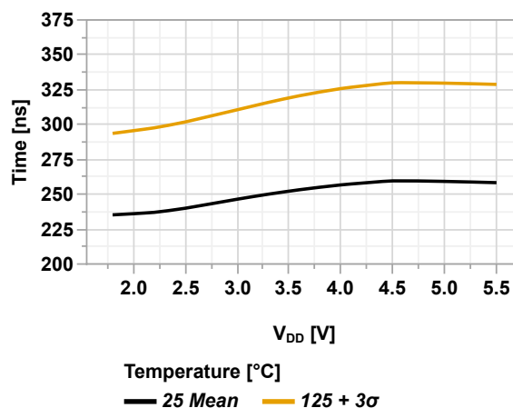
Figure 49-106. Rising Edge Response Time vs. V_{DD} ( V_{CM} = V_{DD}/2 , SP[1:0] = 0x3)
