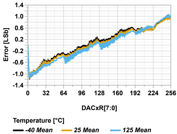
Figure 49-119. INL vs. DAC Code ( V_{REF} = V_{DD} = 3.0V )
