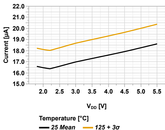
Figure 49-30. I_{PD} HLVD vs. V_{DD}
