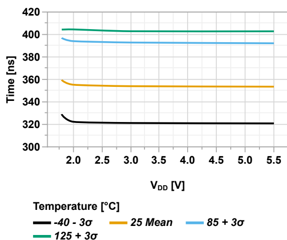
Figure 49-41. Minimum Reset Pulse Width vs. V_{DD}
