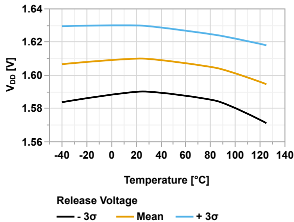
Figure 49-46. POR Release Voltage vs. Temperature
