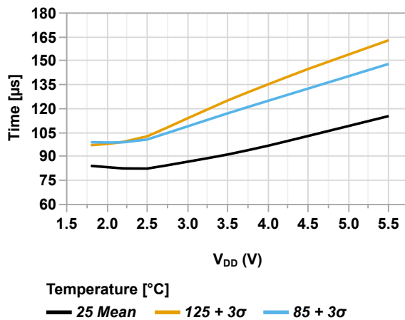
Figure 49-33. Wake-up Time (COSC[2:0] = 'b101, FOSC = 31 kHz, VREGPM[1:0] = 'b11 = ULP + Extended Temperature Range) vs. V_{DD}
