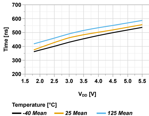
Figure 49-122. Rising Edge Response Time vs. V_{DD}
