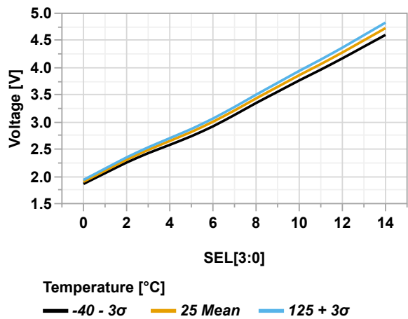
Figure 49-58. HLVD Negative Edge SEL[3:0] vs. Temperature
