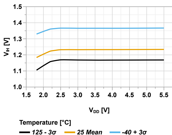
Figure 49-70. Input Pin with SMBus - Maximum V_{IH} vs. V_{DD}
