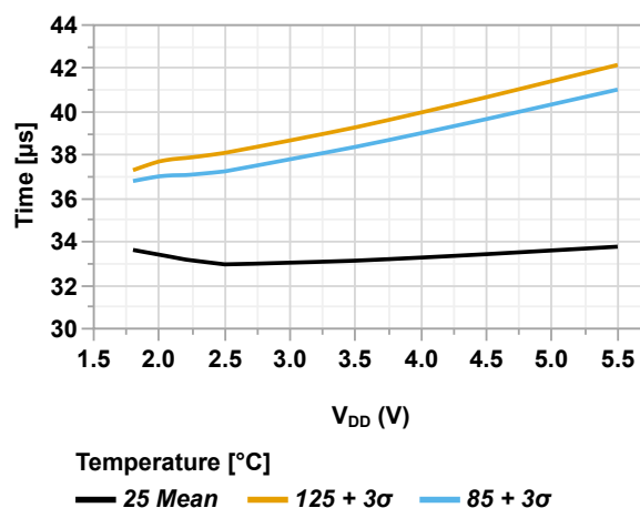
Figure 49-38. Wake-up Time (COSC[2:0] = 'b110, OSCFRQ = 16 MHz, VREGPM[1:0] = 'b01 = LP) vs. V_{DD}
