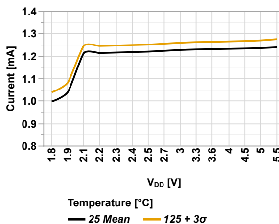
Figure 49-4. Active Power Consumption vs. V_{DD} (RSTOSC[2:0] = 'b110, OSCFRQ = 16 MHz, PMDx = 0xFF)
