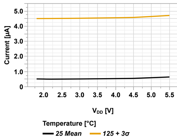
Figure 49-15. I_{PD} Base (VREGPM[1:0] = 'b10 = ULP) vs. V_{DD}
