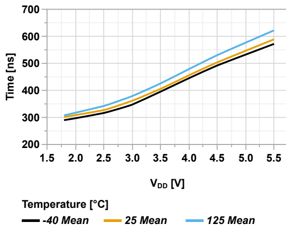
Figure 49-121. Falling Edge Response Time vs. V_{DD}
