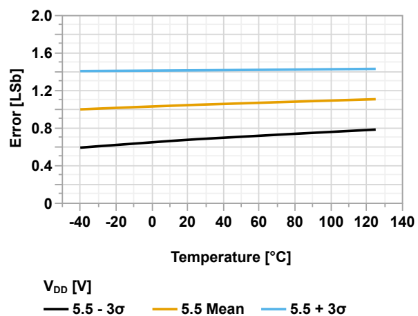
Figure 49-114. Gain Error vs. Temperature ( V_{REF} = V_{DD} = 5.5V )
