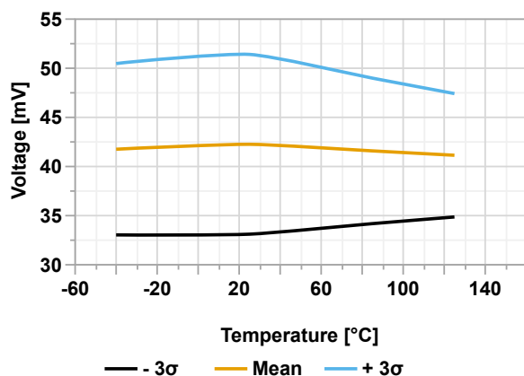
Figure 49-52. BOR Hysteresis (BORV[1:0] = 0x0) vs. Temperature
