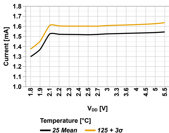
Figure 49-7. Active Power Consumption vs. V_{DD} (RSTOSC[2:0] = 'b111, FEXTOSC[3:0] = 'b0011, HS = 16 MHz, PMDx = 0x00)
