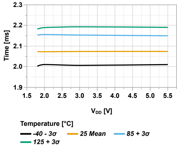
Figure 49-57. WWDT Time-Out Period over V_{DD} and Temperature (PS[4:0] = 0x01)
