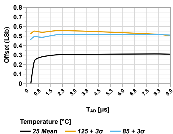
Figure 49-95. Offset Error vs. T_{AD} ( V_{REF+} = 3.0V External, V_{DD} = 3.0V , CPON = 1)
