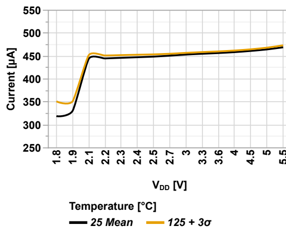
Figure 49-4. Active Power Consumption vs. V_{DD} (RSTOSC[2:0] = 'b110, OSCFRQ = 16 MHz, PMDx = 0xFF)
