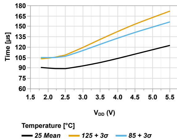
Figure 49-32. Wake-up Time (COSC[2:0] = 'b110, OSCFRQ = 16 MHz, VREGPM[1:0] = 'b11 = ULP + Extended Temperature Range) vs. V_{DD}
