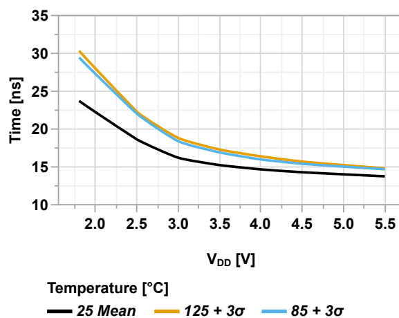
Figure 49-63. Rise Time (SLRxn = 0) vs. V_{DD}
