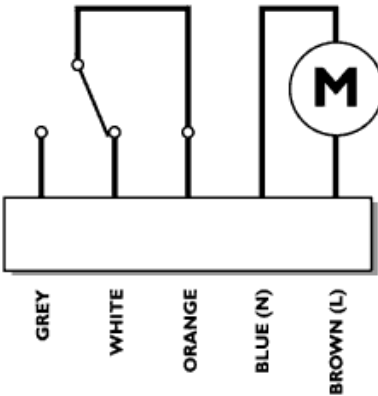
Wiring Diagram HPA2C
