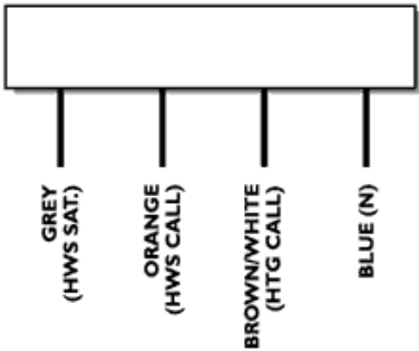
Wiring Diagram HSA3
