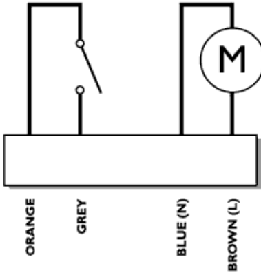
Wiring Diagram HSA3
