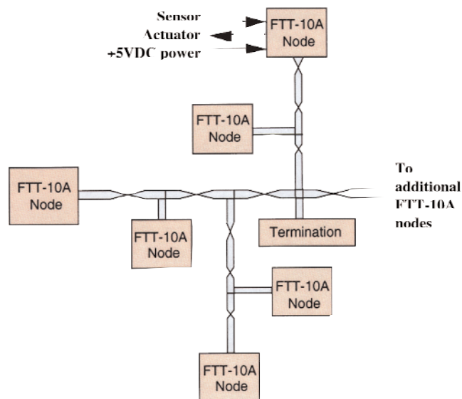
FTT-10A System Block Diagram
