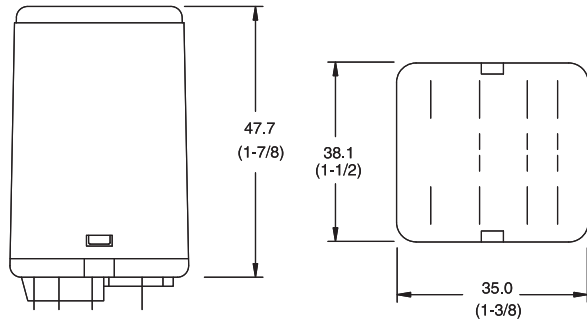
700-HJ Relay
