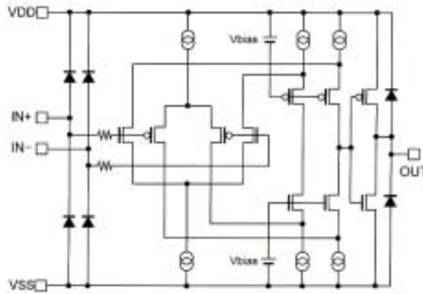
Fig.1 Simplified schematic
