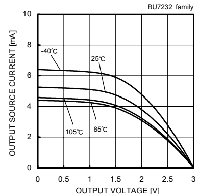
Fig.9 Output Source Current – Output Voltage
