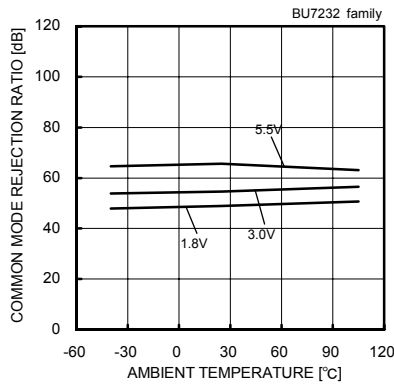
Fig.19 Common Mode Rejection Ratio – Ambient Temperature ( V_{DD}=3[V] )
