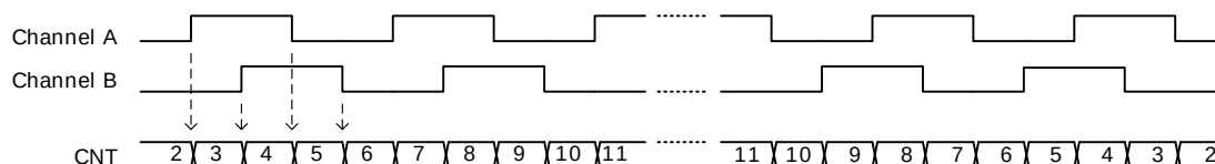
Figure 18.9. TIMER X4 Decoding Mode
