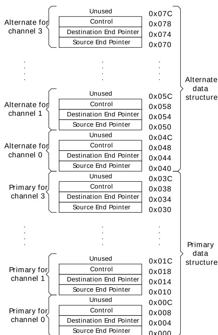
Figure 8.7. Detailed memory map for the 4 channels, including the alternate data structure
