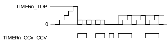
Figure 18.17. TIMER Up-count Frequency Generation
