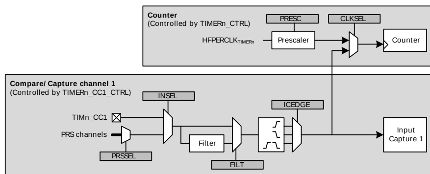
Figure 18.3. TIMER Clock Selection
