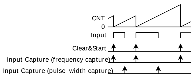
Figure 18.14. TIMER Period and/or Pulse width Capture
