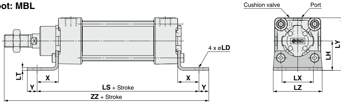
Axial Foot (mm)
