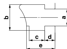
T-slot dimensions
