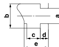
T-slot dimensions
