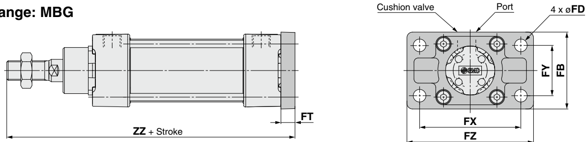
Head Flange (mm)
