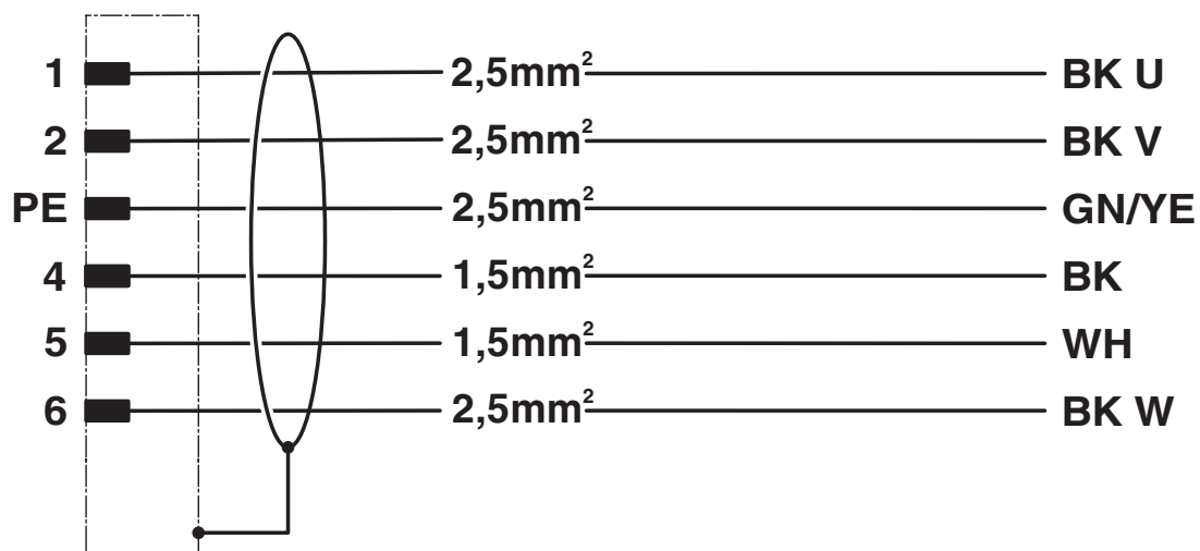
Contact assignment of M23 plugs/sockets
