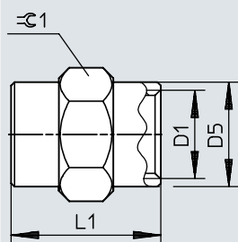
Dimensions – Pipe socket NPFC-S
