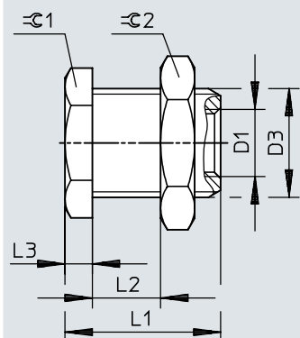
Dimensions – Bulkhead fitting NPFC-H
