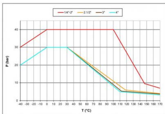
Pressure-temperature chart
