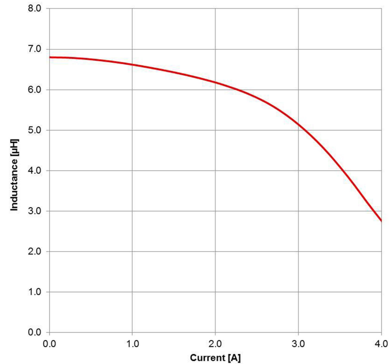
F1 Typical Inductance vs. Current Characteristics:
