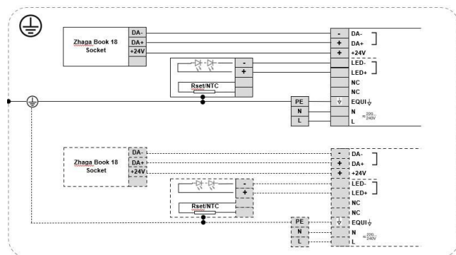
IT DX NFC E Wiring diagram I
